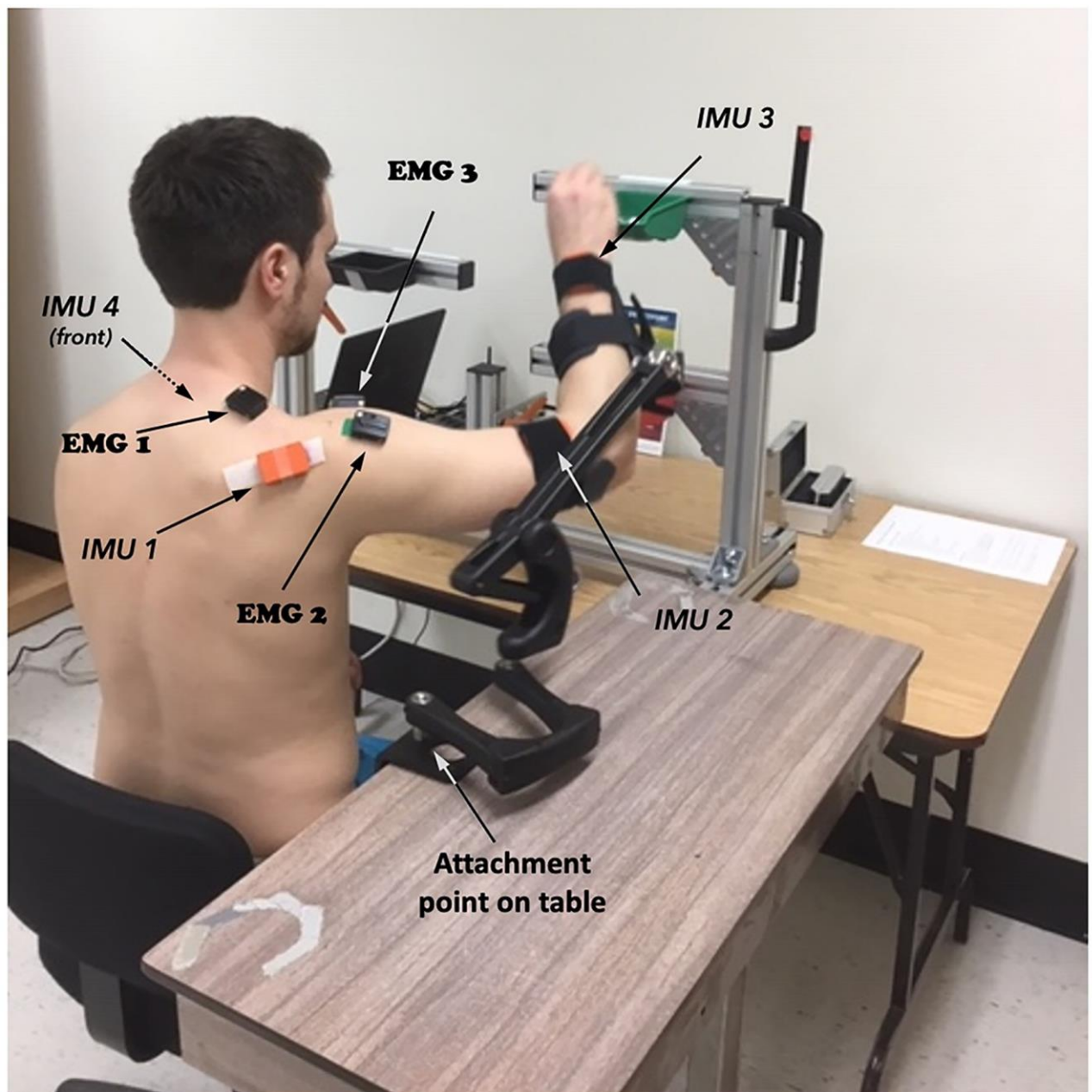
Fig 1. Positions of the three-dimensional dynamic arm support, of the surface electromyographic (EMG) sensors and of the inertial measurement unit (IMU) sensors during the dynamic task. EMG1, upper trapezius; EMG2, middle deltoid; EMG3, anterior deltoid. IMU1, scapula; IMU2, arm; IMU3, distal forearm, IMU4 (not shown on the figure), sternum.
