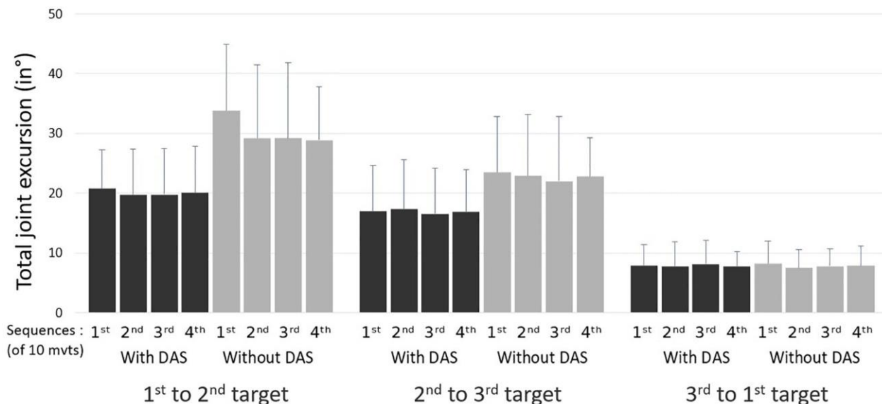
Fig 6. Mean total shoulder elevation excursion (in degrees; with standard deviation) during the dynamic task with and without the dynamic arm support (3D-DAS) (n = 15).
